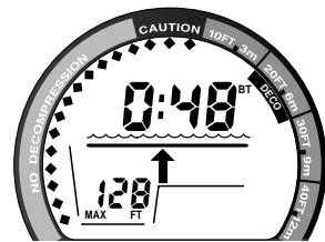
Fig. 34 - Deco Stop Alt #1
