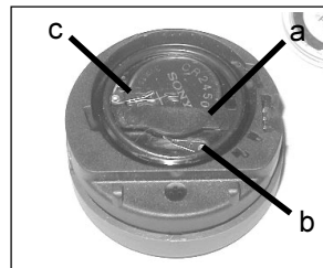
Fig. 46 - Battery Compartment
