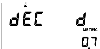
Figure 30a PROGRAMMING MODE (Constant FO2 Mode) (Setting Deco Blend - Depth Benchmark)
