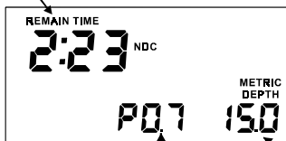
FIGURE 13 PRE DIVE PREDICTION Constant PO2 Mode
