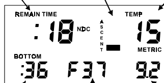
Figure 8 DIVE MODE Primary Screen Constant PO 2 Mode
