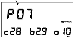
Figure 7 SURFACE DISPLAY Alternate Screen Constant PO 2 Mode With Residual Nitrogen
