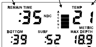
Figure 35 LOGBOOK MODE (Primary Screen)
