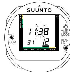
Fig. 4.15 TIME SETTING
